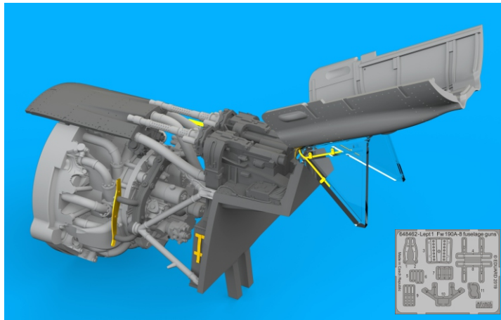
648 649 Fw 190F-8 fuselage guns
