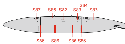
220gal/1.000 l auxiliary fuel tank (right)
